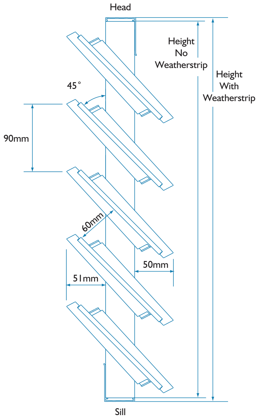
152mm Fixed Louvre
