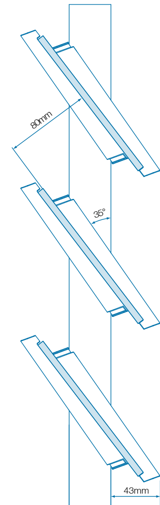
152mm Louvre 80mm Restricted Opening
