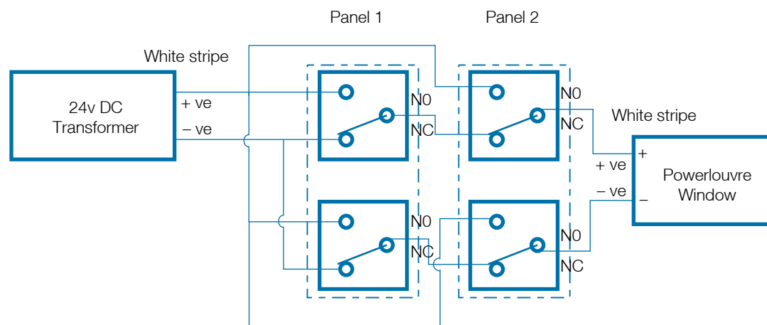
Twin Switch Panel Wiring
