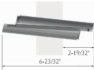
Altair® Stronghold 6" Clip
