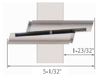
Altair® Stronghold 4" Clip
